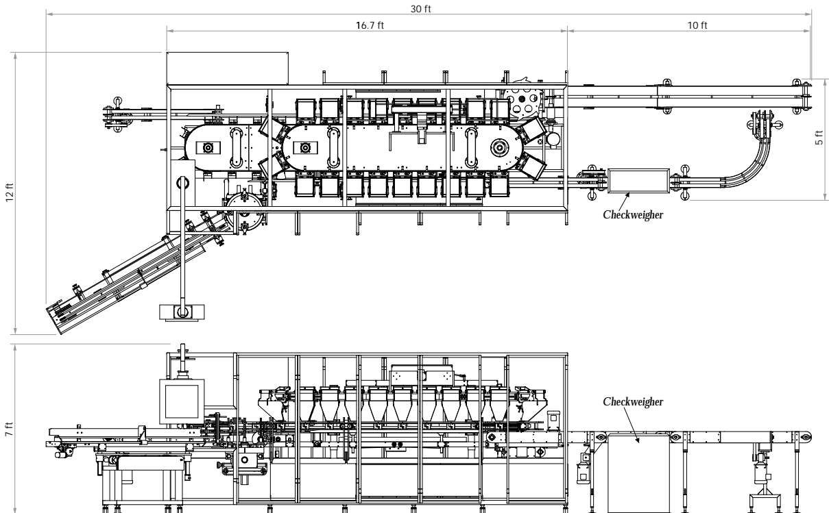
Product Streaming Delivery System
