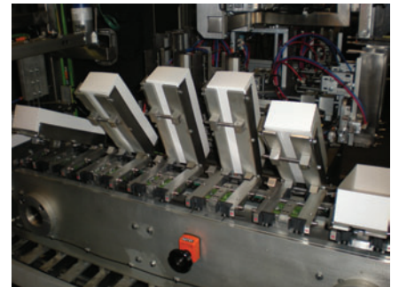
Tilt-Up Tray Pockets for Product Loading
