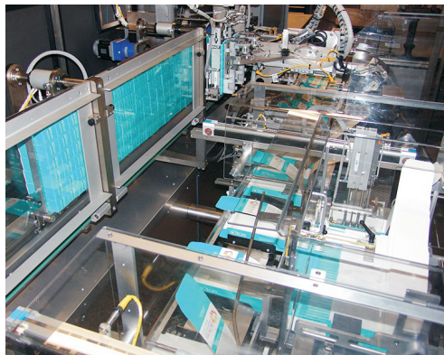
Vertical stacker (left) and tray placing system (right)
