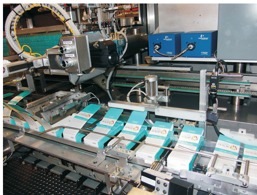
Servo driven pick and place unit and tray cell chain
