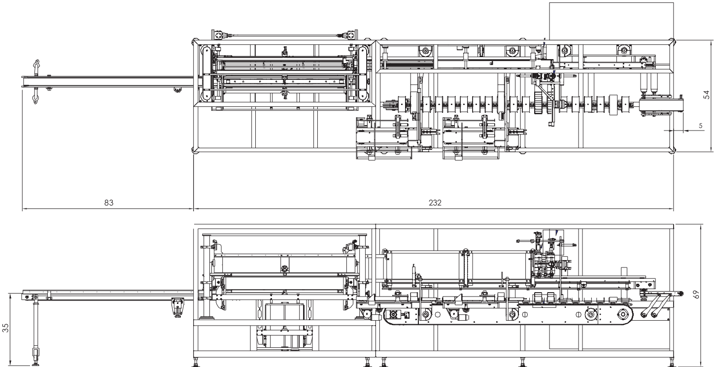
Vertical stacker (left) and tray placing system (right)
